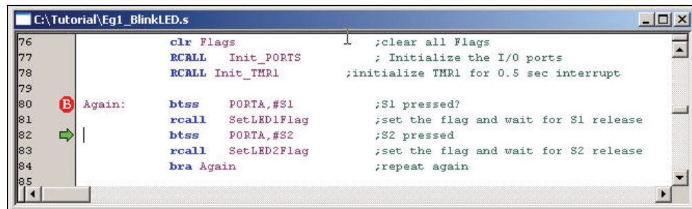
FIGURE 2-17: SETTING BREAKPOINT
